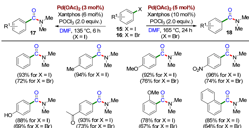
Scheme 7. Pd-catalyzed aminocarbonylation of aryl iodides 15 and bromides 16 with DMF as a CO source, proposed in 2011 by Bhanage et al. [33]. For each carbonylated product 17–18 , the yield after column chromatography purification is reported in brackets.
