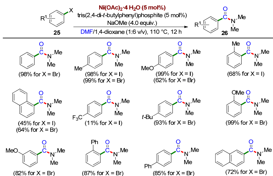
Scheme 10. Ni-catalyzed aminocarbonylation of aryl iodides/bromides 25 , using DMF as the source of CO and N,N -dimethylamino groups, reported in 2007 by Lee and co-workers [37]. For each carbonylated product 26 , yield after column chromatography purification was reported in brackets.
