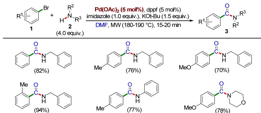
Scheme 2. Pd-catalyzed aminocarbonylation of aryl bromides 1 with amines 2 , in the presence of DMF as a CO surrogate, reported in 2002 by Hallberg, Alterman et al. [28]. For each carbonylated product 3 , yield after column chromatography purification was reported in brackets.
