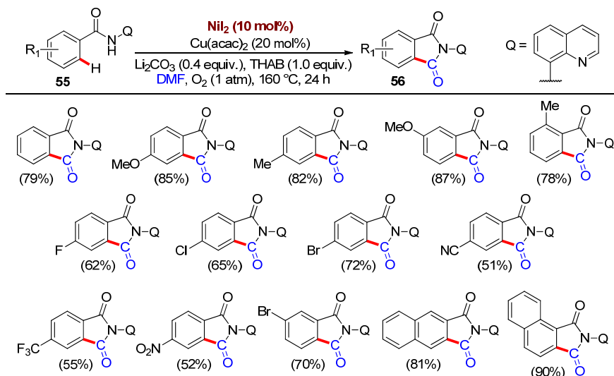
Scheme 21. Synthesis of phthalimides 56 by carbonylative cyclization of aromatic C(sp 2 )-H of amides 55 using DMF as CO surrogate, promoted by the synergistic action of NiI 2 as the main catalyst and Cu(acac) 2 as co-catalyst, reported in 2015 by Ge and co-workers [63]. For each heterocyclic carbonylated product, yield after column chromatography purification is reported in brackets.
