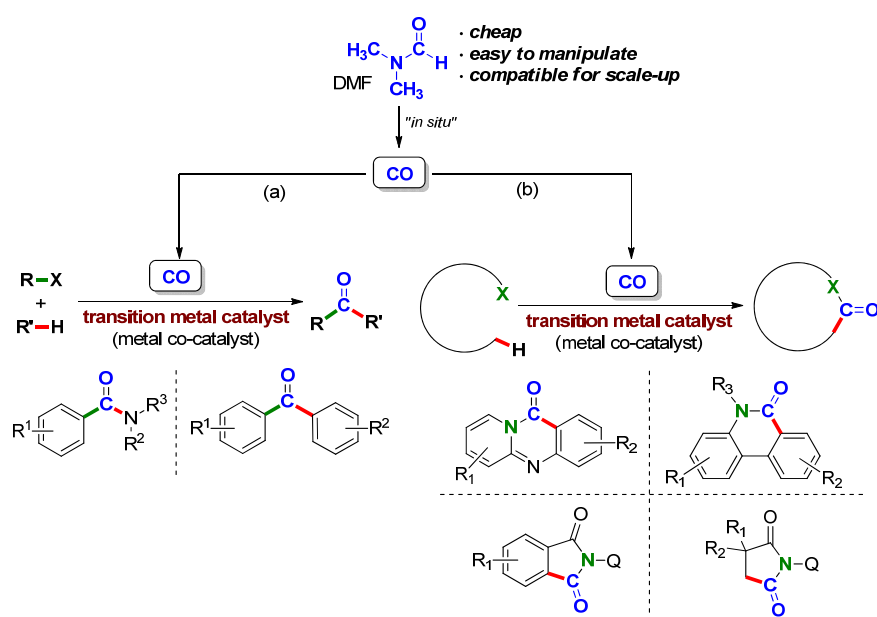
Scheme 1. Transition metal-catalyzed carbonylation reactions involving DMF as CO surrogate: (a) general scheme for the synthesis of carbonyl-containing molecules; (b) application to the synthesis of heterocycles.
