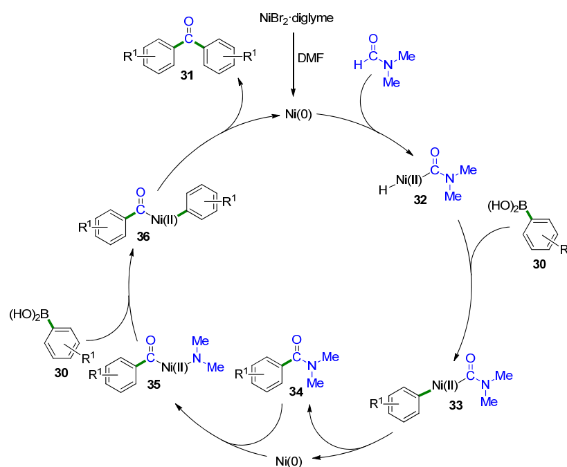
Scheme 13. Proposed reaction mechanism for the Ni-catalyzed carbonylative homo-coupling of aryl boronic acids 30 with DMF as a CO surrogate, reported in 2017 by Lu, Liu and co-workers [39].
