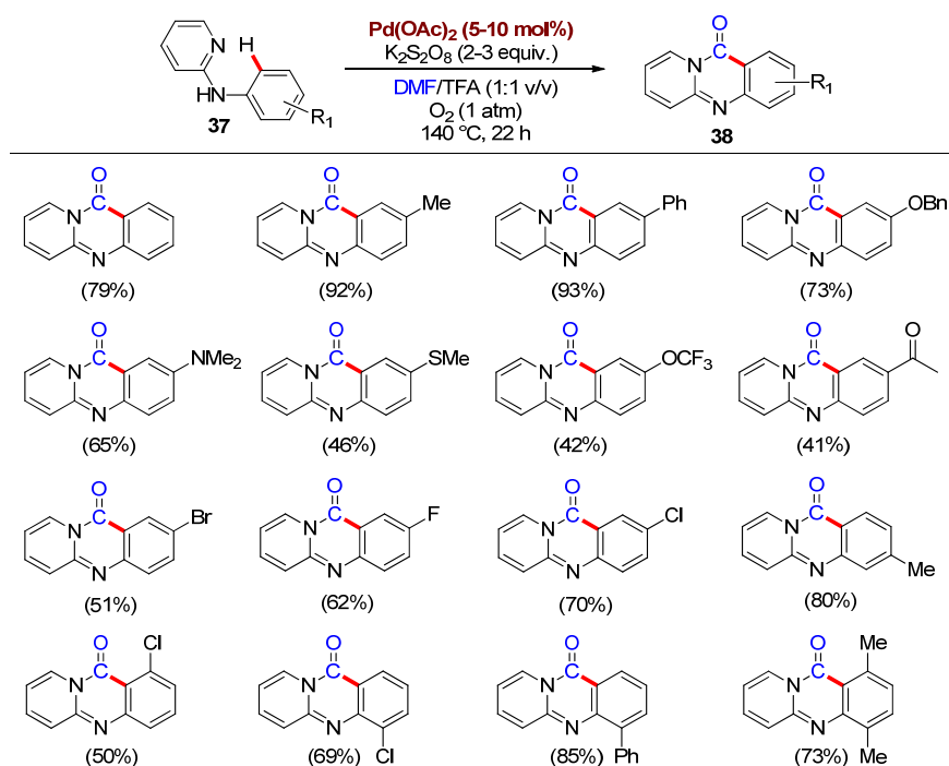
Scheme 14. Pd-catalyzed carbonylative cyclization of N -arylpyridin-2-amines 37 using DMF as a CO surrogate for the synthesis of quinazolinones 38 , reported in 2015 by Wu and co-workers [41]. For each heterocyclic carbonylated product, the yield after chromatographic purification is reported in brackets.
