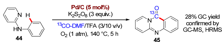
Scheme 17. Pd/C-catalyzed carbonylative cyclization of N -phenyl pyridin-2-amine 44 using carbonyl - 13 C-labeled DMF: synthesis of 11 H -pyrido[2,1- b ]quinazolin-11-one-11- 13 C 45 .
