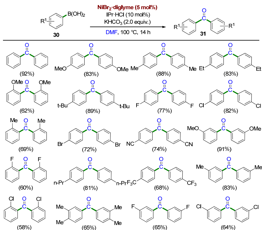
Scheme 12. Ni-catalyzed carbonylative homo-coupling of aryl boronic acids 30 with DMF as a CO surrogate, reported in 2017 by Lu, Liu and co-workers [39]. For each carbonylated product 31 , yield after column chromatography purification is reported in brackets.
