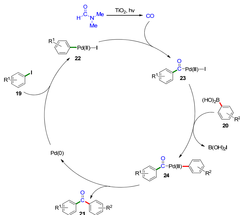
Scheme 9. Simplified proposed reaction mechanism for the Pd-catalyzed photocatalytic carbonylative Suzuki–Miyaura coupling of aryl iodides 19 with aryl boronic acids 20 , reported in 2017 by Li et al. [34].
