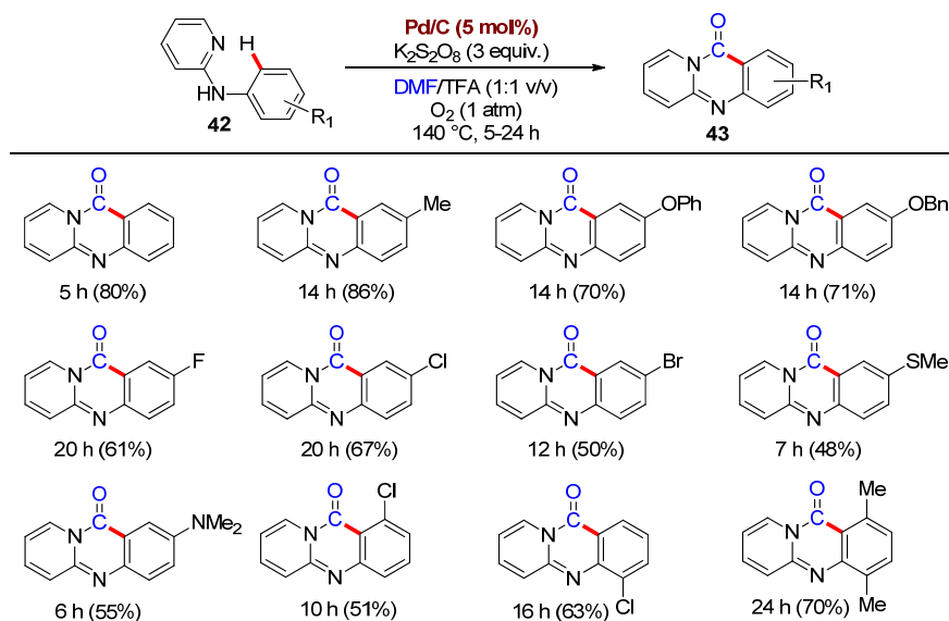
Scheme 16. Synthesis of quinazolinones 43 through carbonylative cyclization of N -arylpyridin-2-amines 42 with DMF as a CO surrogate catalyzed by Pd/C, developed in 2015 by Wu et al. [53]. For each heterocyclic product, reaction time and yield after chromatographic purification (in brackets) are reported.
