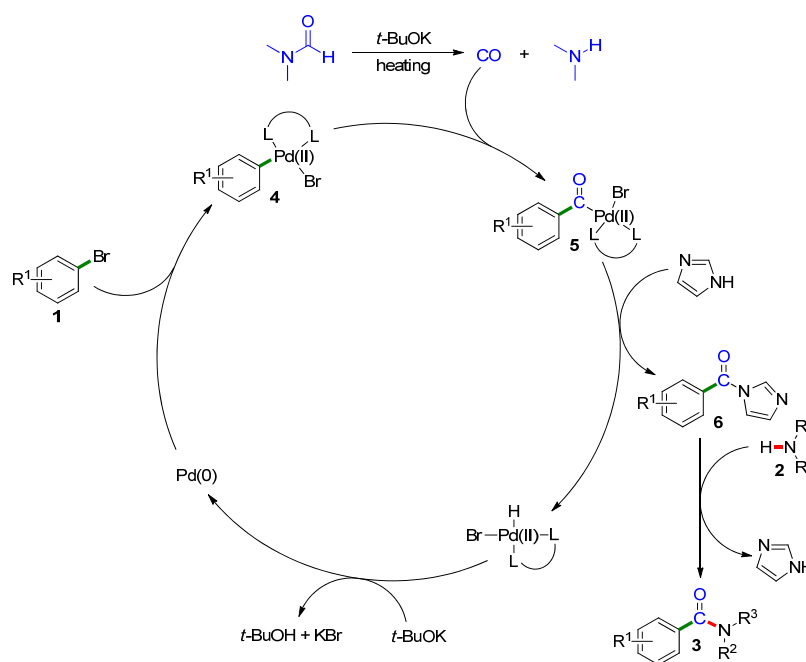
Scheme 3. Proposed reaction mechanism for the Pd-catalyzed aminocarbonylation of aryl bromides 1 with amines 2 using DMF as a CO surrogate, reported in 2002 by Hallberg, Alterman et al. [28].
