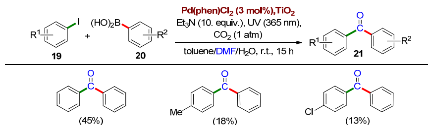
Scheme 8. Pd-catalyzed photocatalytic carbonylative Suzuki–Miyaura coupling of aryl iodides 19 with aryl boronic acids 20 , achieved in 2017 by Li et al. [34]. For each carbonylated product 21 , yield is reported in brackets.
