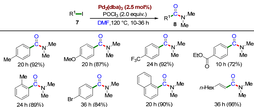
Scheme 4. Pd-catalyzed aminocarbonylation of aryl and alkenyl iodides 7 , in the presence of DMF as a source of CO and N,N -dimethylamino groups, reported in 2002 by Hiyama, Nozaki et al. [30]. For each carbonylated product 8 , reaction time and yield after column chromatography purification (in brackets) were reported.
