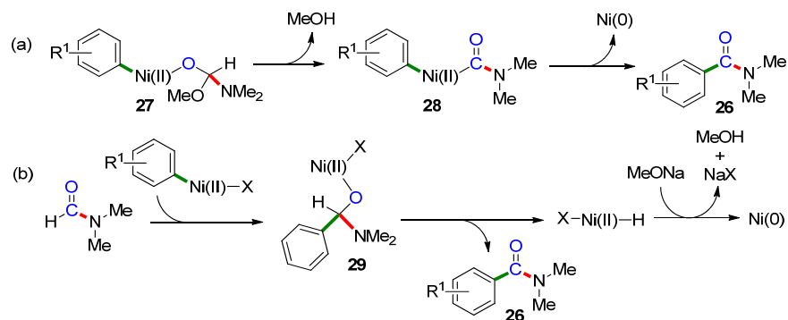
Scheme 11. Simplified proposed reaction mechanism for the Ni-catalyzed aminocarbonylation of aryl iodides/bromides 25 , using DMF as the source of CO and N,N -dimethylamino groups, reported in 2007 by Lee and co-workers [37].
