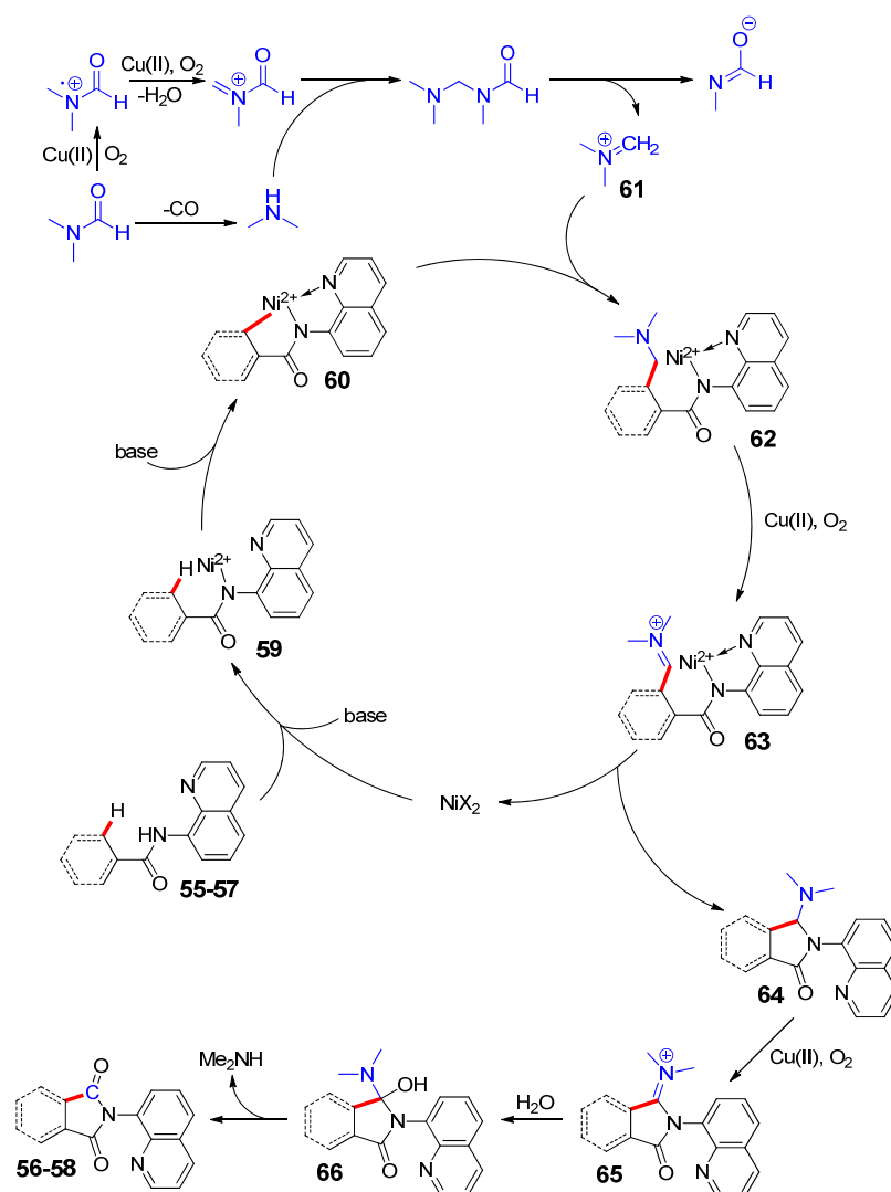
Scheme 23. Proposed reaction mechanism for the synthesis of phthalimides 56 and succinimides 58 by Ni/Cu synergistic catalyzed carbonylative cyclization of aromatic C(sp 2 )-H and aliphatic C(sp 3 )-H bonds of amides 55–57 using DMF as a CO surrogate, reported in 2015 by Ge and co-workers [63].
