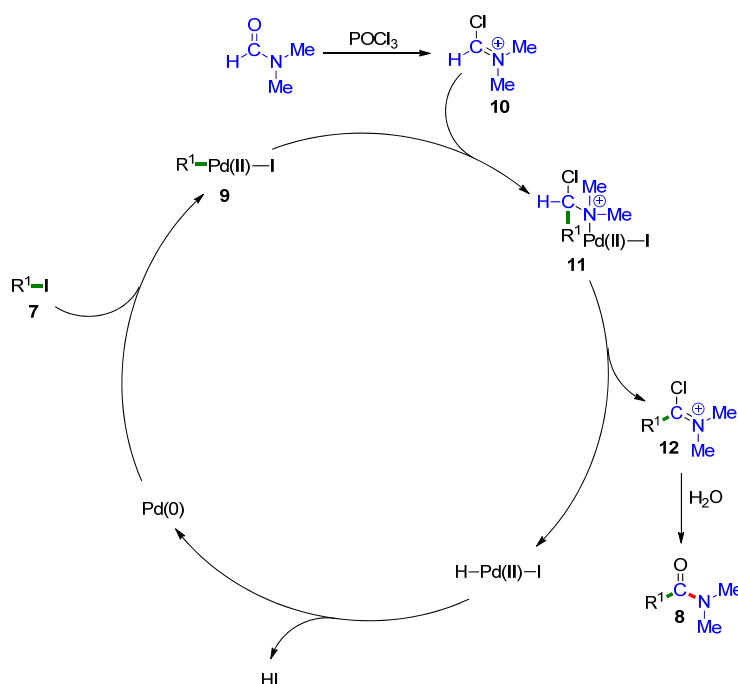
Scheme 5. Proposed reaction mechanism for the Pd-catalyzed aminocarbonylation of aryl and alkenyl iodides 7 , in the presence of DMF as a source of CO and N,N -dimethylamino groups, reported in 2002 by Hiyama, Nozaki et al. [30].
