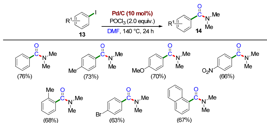
Scheme 6. Pd-catalyzed aminocarbonylation of aryl iodides 13 in the presence of DMF as a source of CO and N,N -dimethylamino groups, investigated in 2008 by Bhanage et al. [32]. For each carbonylated product 14 , the yield after column chromatography purification is reported in brackets.
