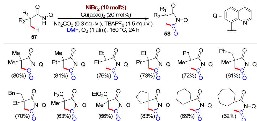
Scheme 22. Synthesis of succinimides 58 by carbonylative cyclization of aliphatic C(sp 3 )-H bonds of amides 57 using DMF as a CO surrogate, promoted by the synergistic action of NiBr 2 as the main catalyst and Cu(acac) 2 as co-catalyst, reported in 2015 by Ge and co-workers [63]. For each heterocyclic carbonylated product, yield after column chromatography purification is reported in brackets.
