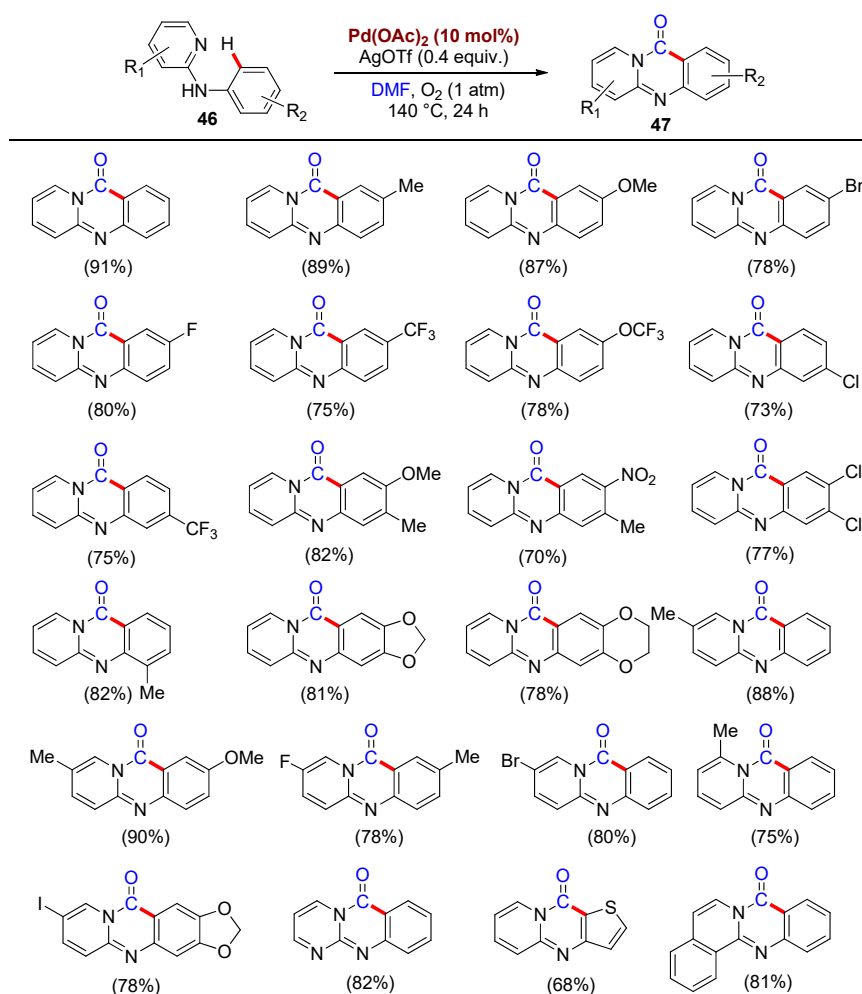
Scheme 18. Synergistic Pd/Ag-catalyzed carbonylative cyclization of N -arylpyridin-2-amines 46 using DMF as a CO surrogate for the synthesis of quinazolinones 47 , reported in 2016 by Das et al. [58]. For each heterocyclic carbonylated product, the yield after column chromatography purification is reported in brackets.
