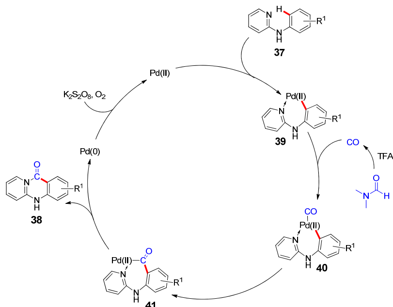
Scheme 15. Proposed reaction mechanism for the synthesis of quinazolinones 38 by Pd-catalyzed carbonylative cyclization of N -arylpyridin-2-amines 37 using DMF as a CO surrogate, reported in 2015 by Wu and co-workers [41].
