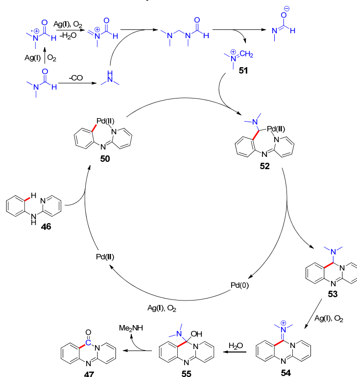
Scheme 20. Proposed reaction mechanism for the synthesis of quinazolinones 47 and phenanthridinones 49 by a Pd/Ag synergistic catalyzed carbonylative cyclization of N -arylpyridin-2-amines and N -methyl 2- arylanilines using DMF as a CO surrogate, reported in 2016 by Das et al. [58].
